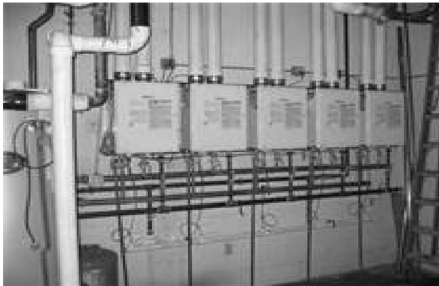
On-Demand Water Heaters in Series
