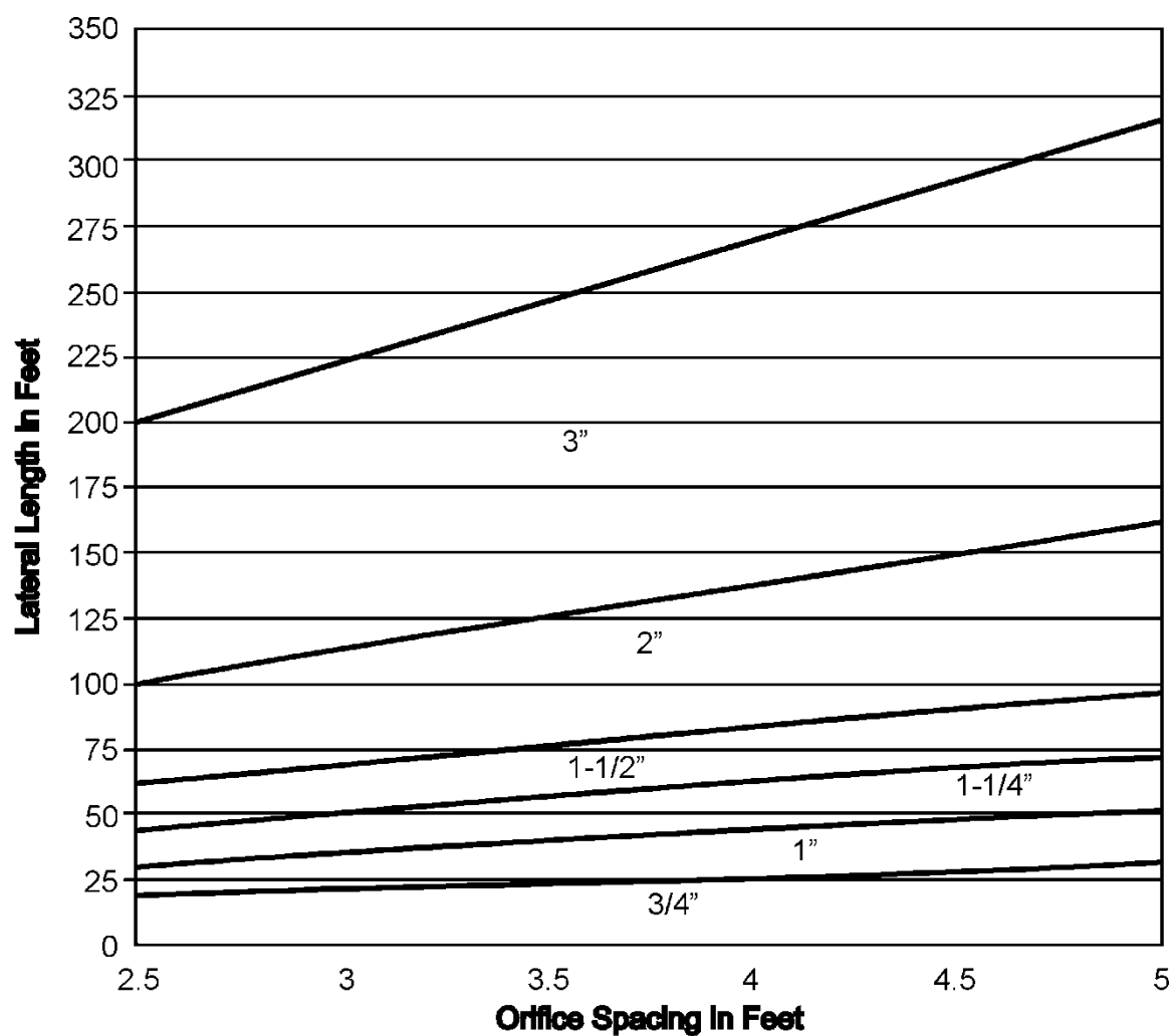
Fig. A-3a. Minimum lateral diameter based on orifice spacing for 3/16 in. diameter orifices (Wisc. Dept. Of Commerce, 1999)
