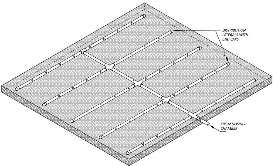
Figure 20.F Central Manifold Distribution Network
