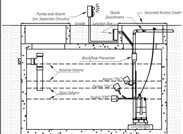
DOSE TANK
