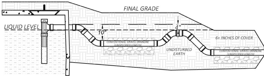
SERIAL SYSTEM DETAIL
