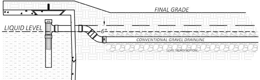
LEVEL FIELD SYSTEM DETAIL
