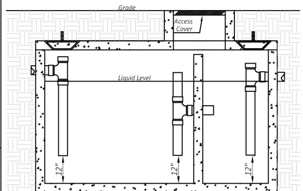
GREASE TRAP
