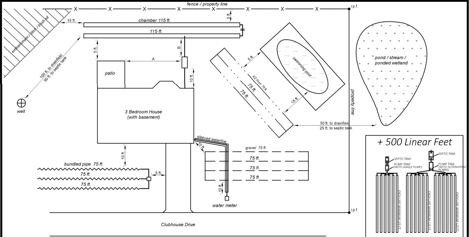
SERIAL SYSTEM DETAIL
