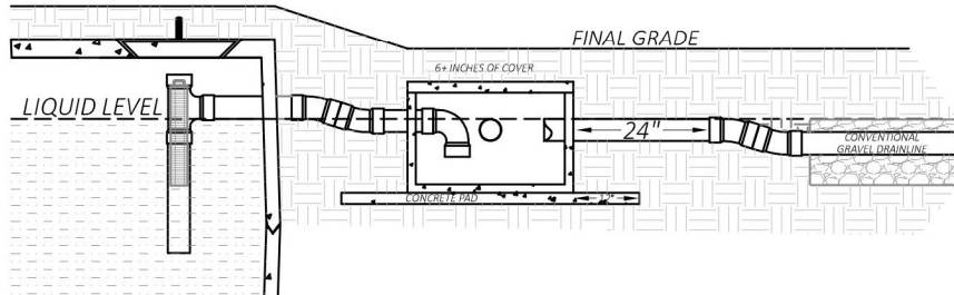
EQUAL DISTRIBUTION SYSTEM DETAIL
