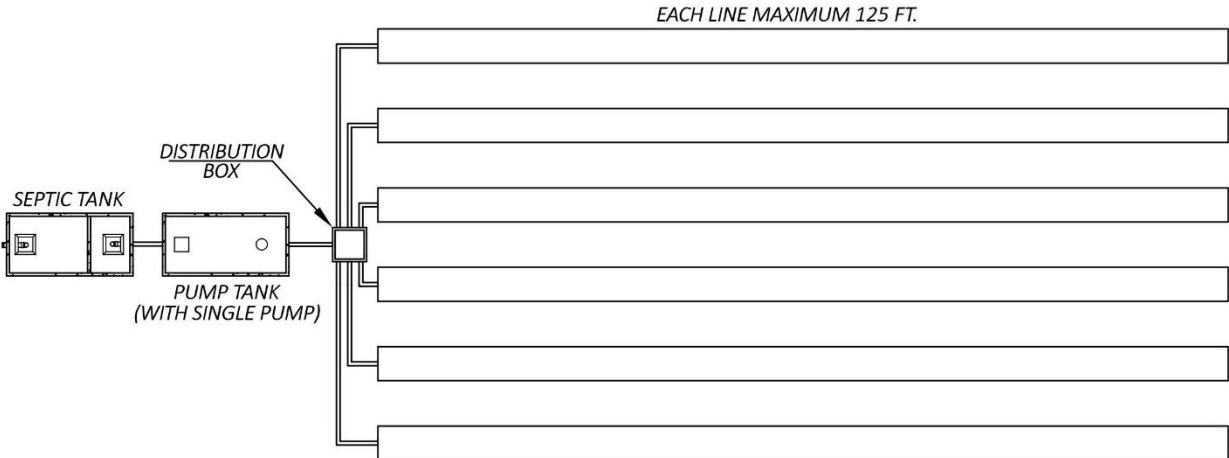
Figure 14.E Criteria for Drainfields >1000
